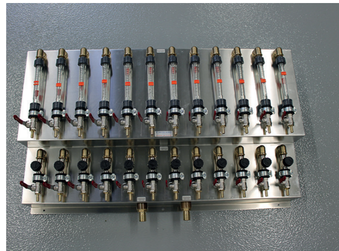
12-WAY MULTIPLE DISTRIBUTOR WITH REGULATION VALVE
