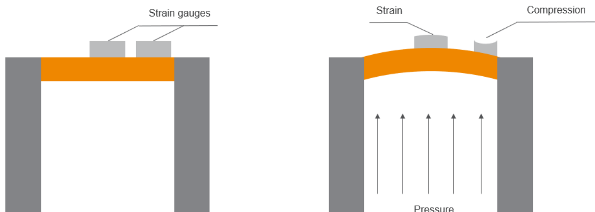
Figure 2: Functional principle of a thin-film coated strain gauge
