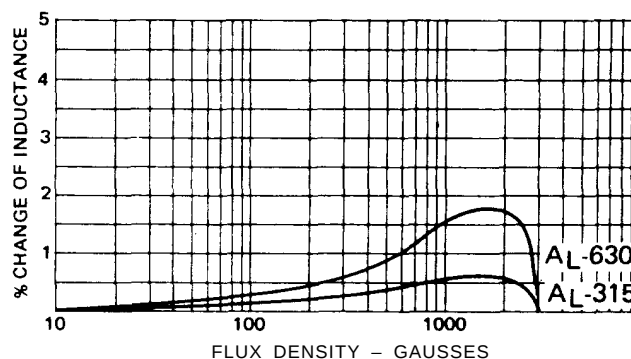
Figure 3 — Ferrite Pot Core
