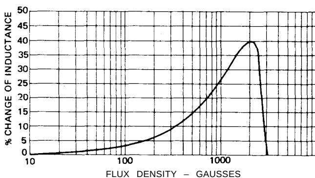
Figure 2 — Ferrite Toroid
