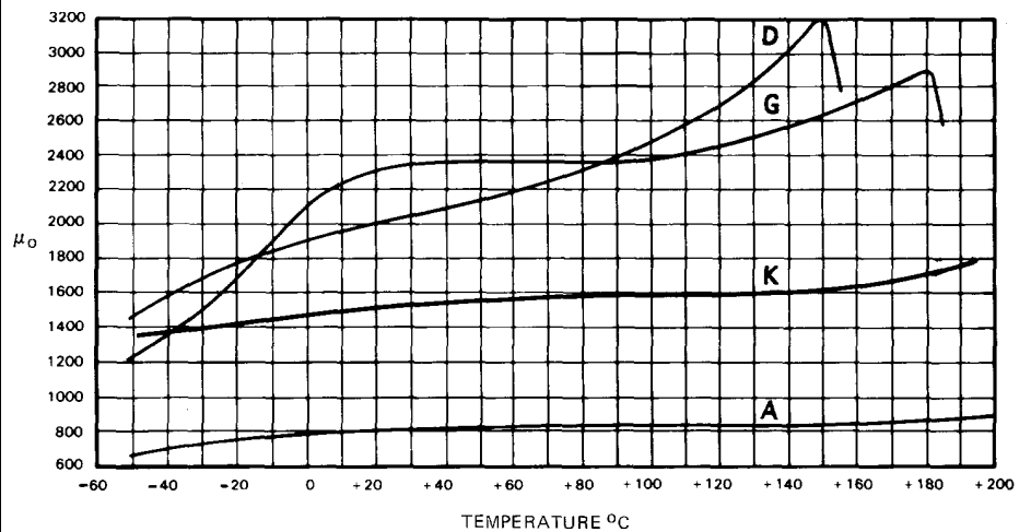
Figure 1 — Ferrite Toroids Initial Permeability ( \mu_0 ) Vs. Temperature
