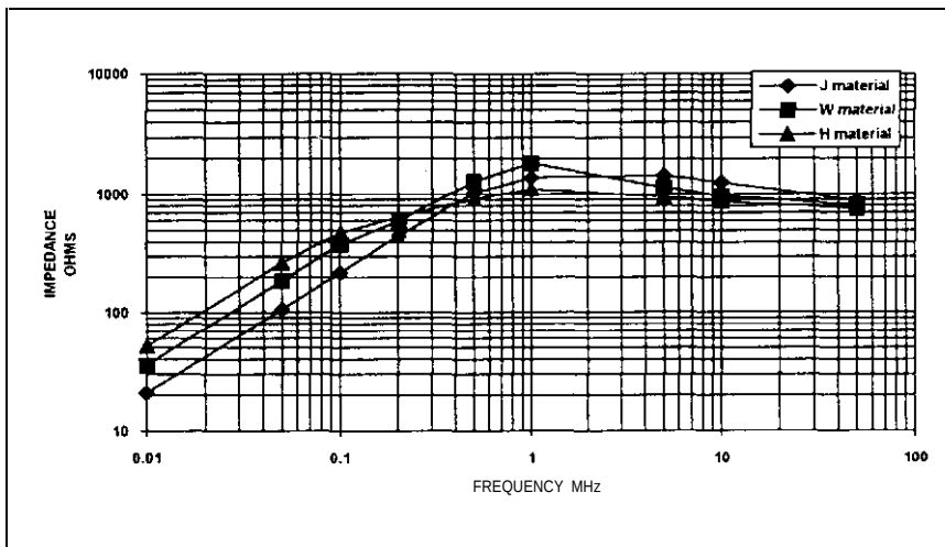
Figure 8. Total Impedance vs Frequency.
