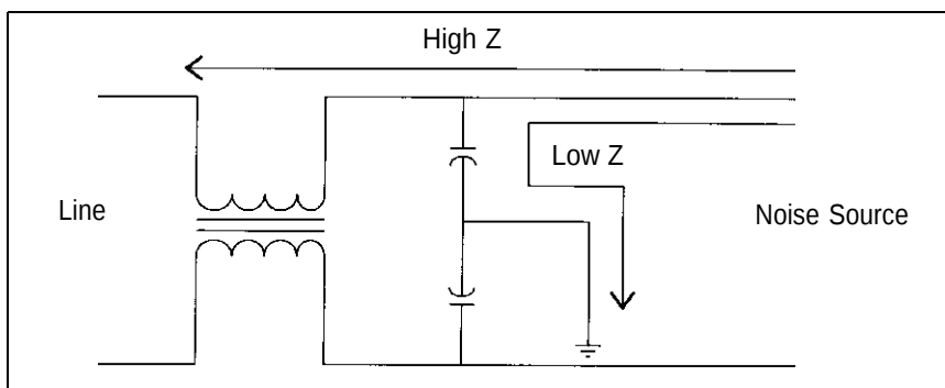
Figure 2. Common Mode Filter.
