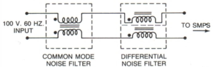
FIGURE 1: SCHEMATIC OF AN EMI FILTER
