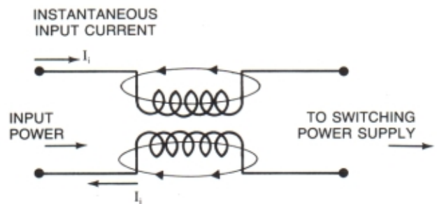
2a: REACTION TO INSTANTANEOUS INPUT CURRENT
