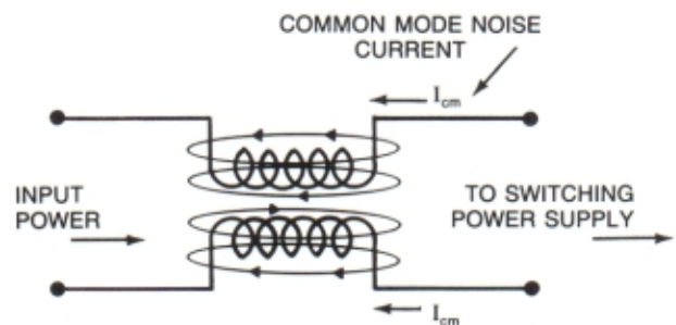
2b: REACTION TO CMN CURRENT
