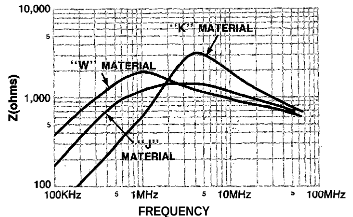
FIGURE 5: IMPEDANCE VS FREQUENCY OF FERRITE TOROIDS IN THREE DIFFERENT MATERIALS
