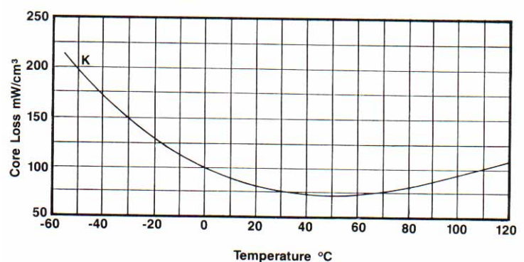
Figure 2 Core Loss vs. Temperature @ 500 kHz, 500 Gauss
