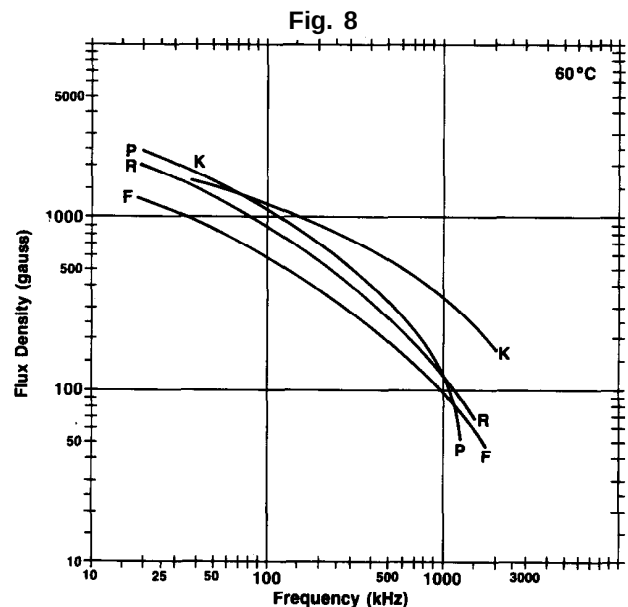
USABLE FLUX DENSITY vs. FREQUENCY @ constant core loss = 100 mW/cm 3
