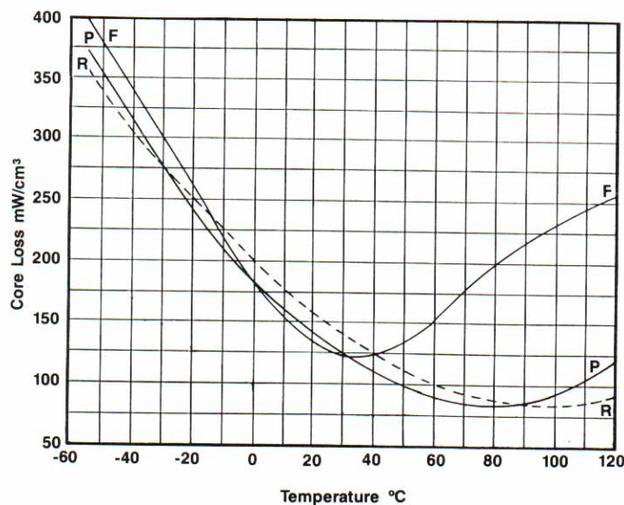
Figure 1 Core Loss vs. Temperature @ 100 kHz, 1K Gauss
