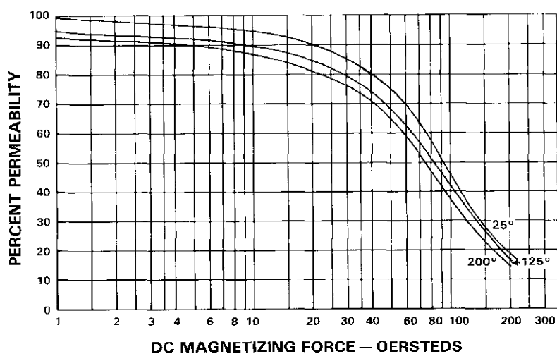
FIG. 10: Kool Mu PERMEABILITY VS. DC BIAS CURVES AT VARIOUS TEMPERATURES
