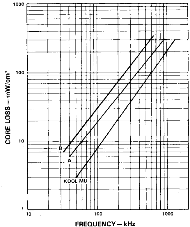
FIG. 7: CORE LOSS CURVES FOR IRON POWDER AND KOOL MU AT FLUX DENSITY OF 100 GAUSS
