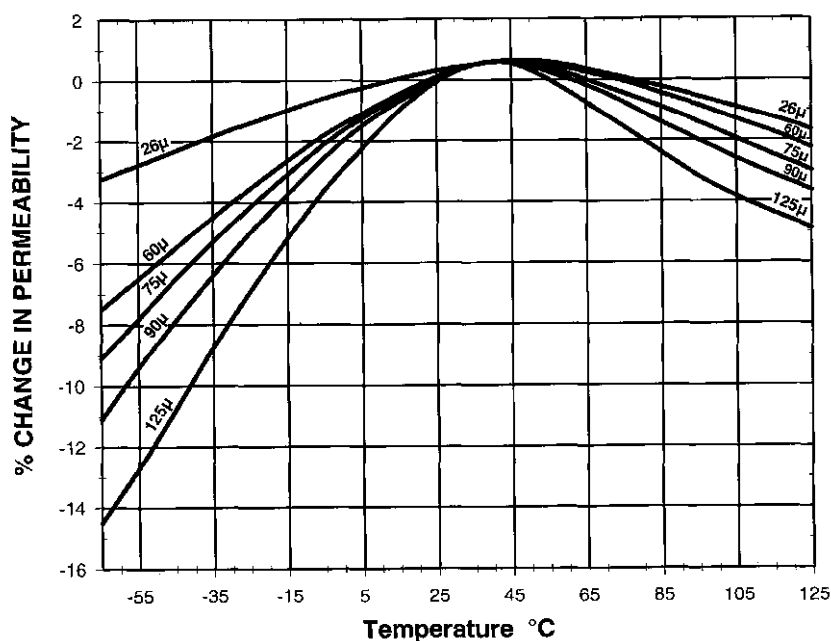
FIG. 9: PERMEABILITY VARIATIONS OVER TEMPERATURE FOR Kool Mu
