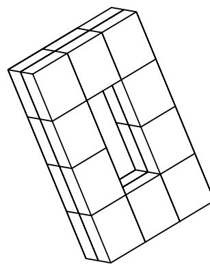
QUANTITY OF 20 4741B BLOCKS A_L = 202 \pm 8\% (26 \mu )
