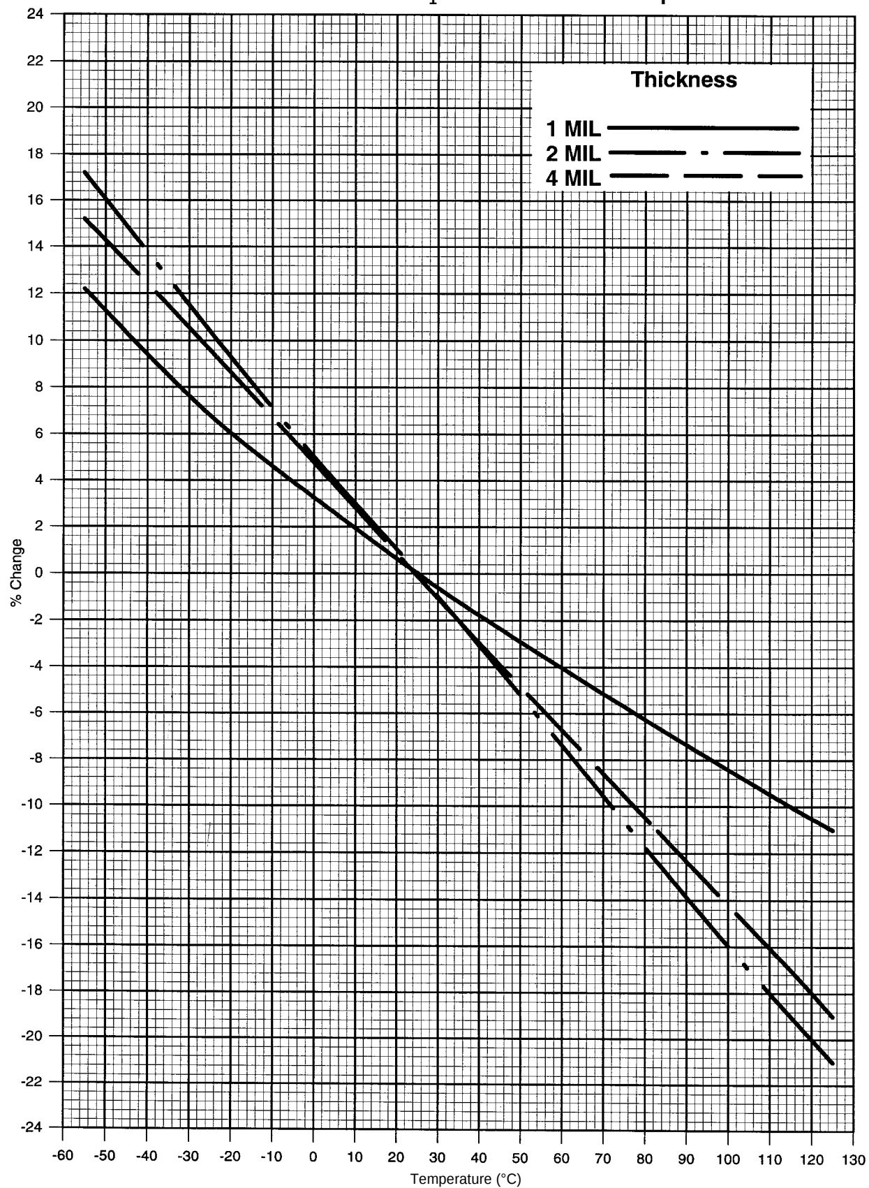
Curve #3: Variation of H_1 of Orthonol with temperature
