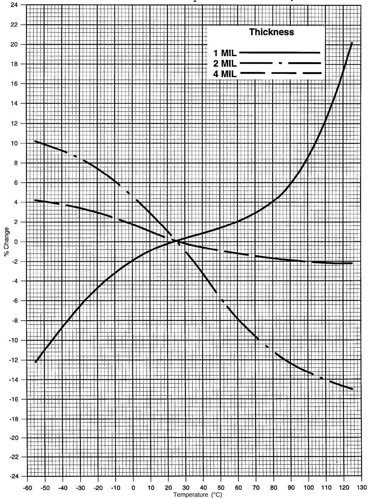
Curve #4: Variation of \delta H_1 of Orthonol with temperature
