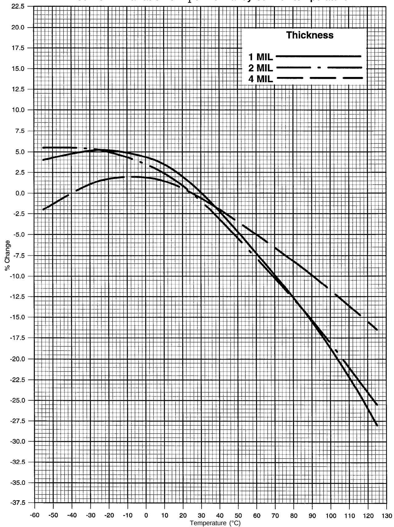
Curve #7: Variation of H_1 of Permalloy 80 with temperature
