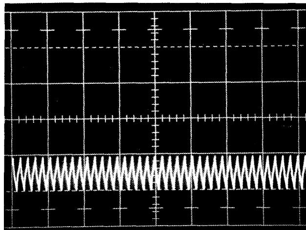
Figure 33 Same as Figure 32 But the Core was Cut and Operating With a Maximum Flux Density Value of B_{\text{operate}} = B_{\text{maximum}} - B_{\text{residual}}
