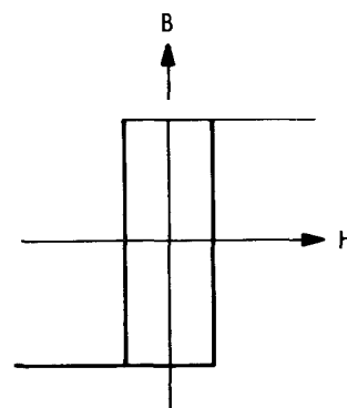
Figure 2 Ideal Square B-H Loop
