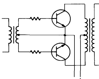
Figure 1 Typical Driven Transistor Inverter
