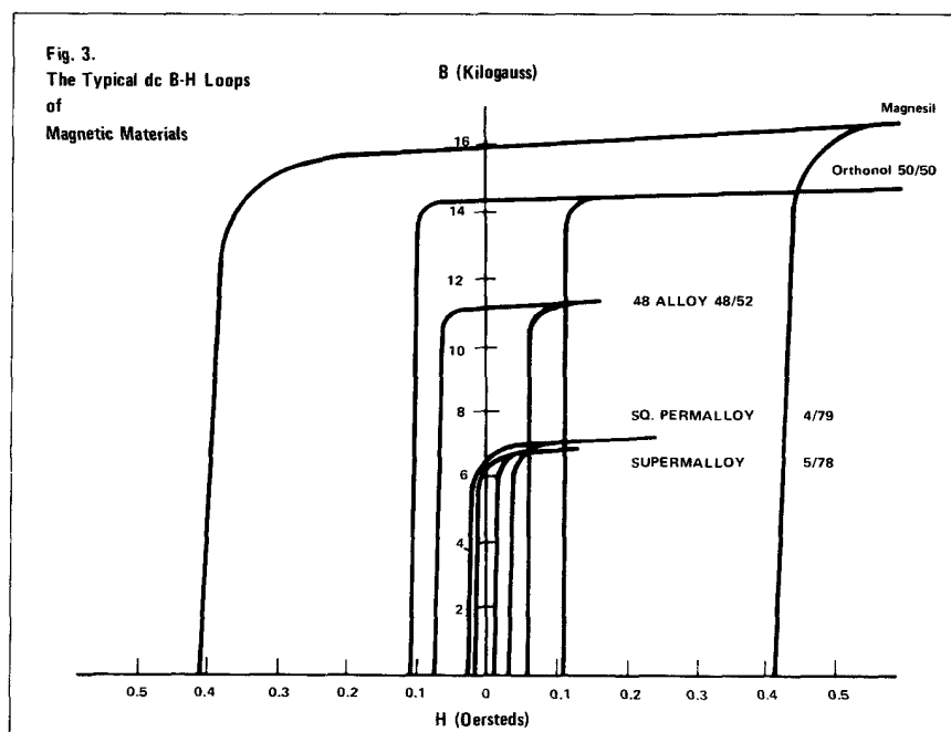
Figure 3 The Typical dc B-H Loops of Magnetic Materials
