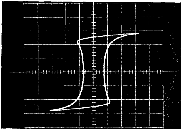
Figure 11 48 Alloy H B-H Loop
