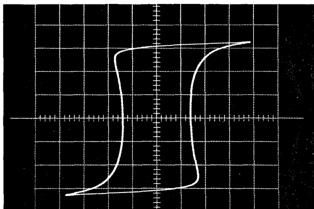
Figure 9 Magnesil K B-H Loop
