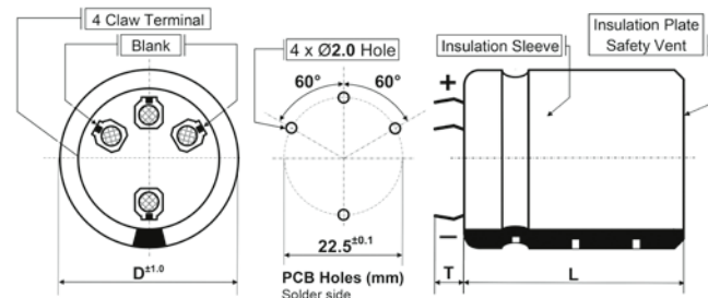
Shape · Form: S (D = 35 ~ 46 mm, long pin T = 6.3 \pm 1.0 mm) X (D = 35 ~ 46 mm, short pin T = 4.0 \pm 1.0 mm)
