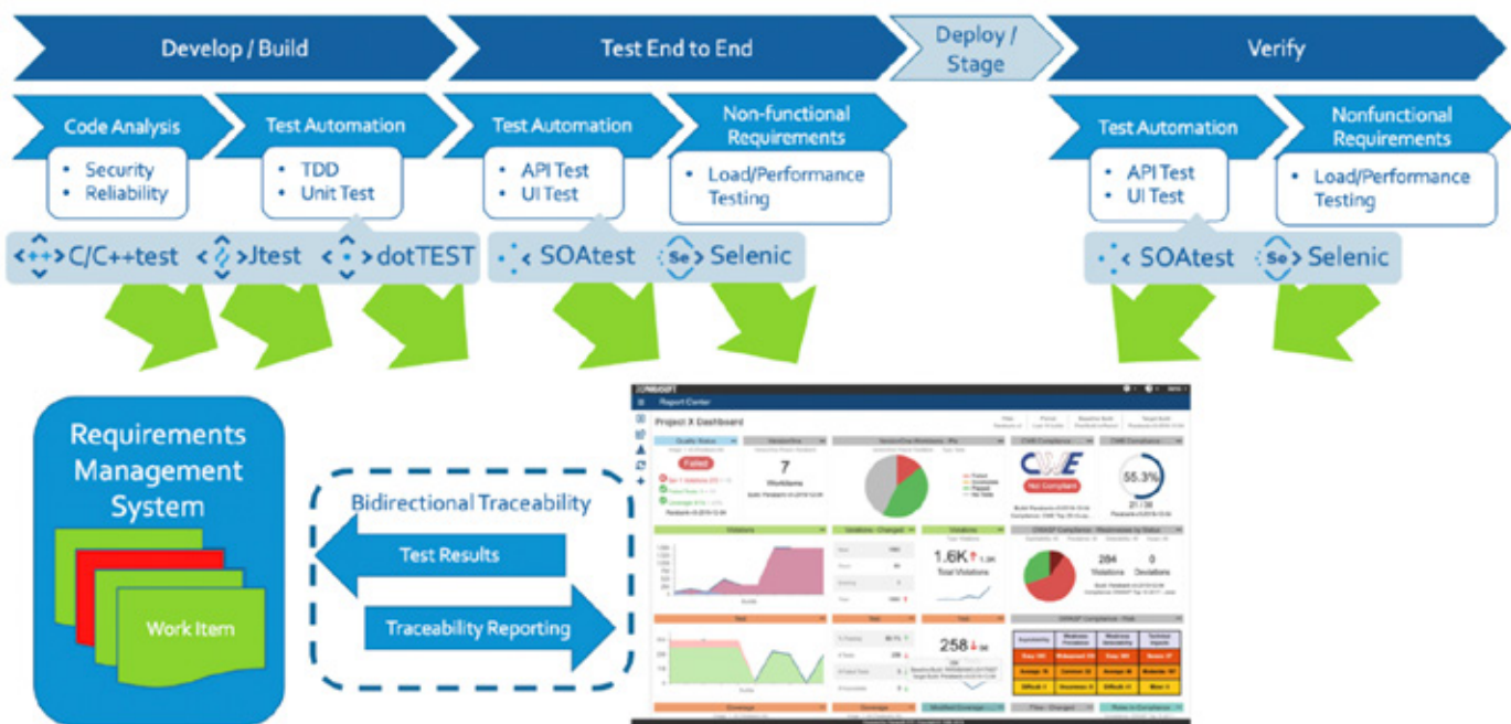
Figure 6: Parasoft provides bidirectional traceability from work items to test cases and test results - both displaying traceability reports with Parasoft DTP as well as reporting results back to the requirements management system.
